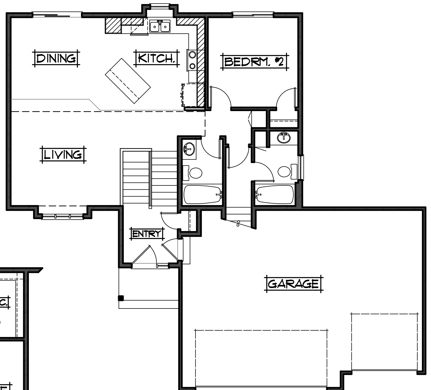
MAIN LEVEL 932 SQ.FT.
